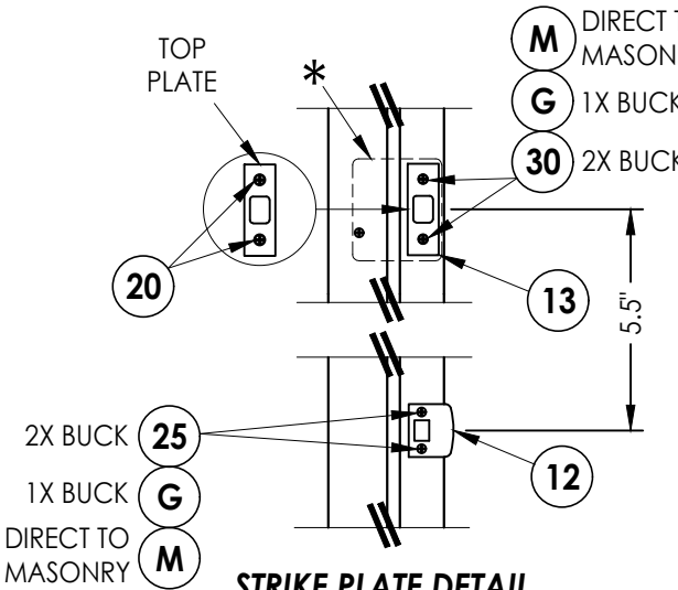
STRIKE PLATE DETAIL SCHLAGE LOCKSET
