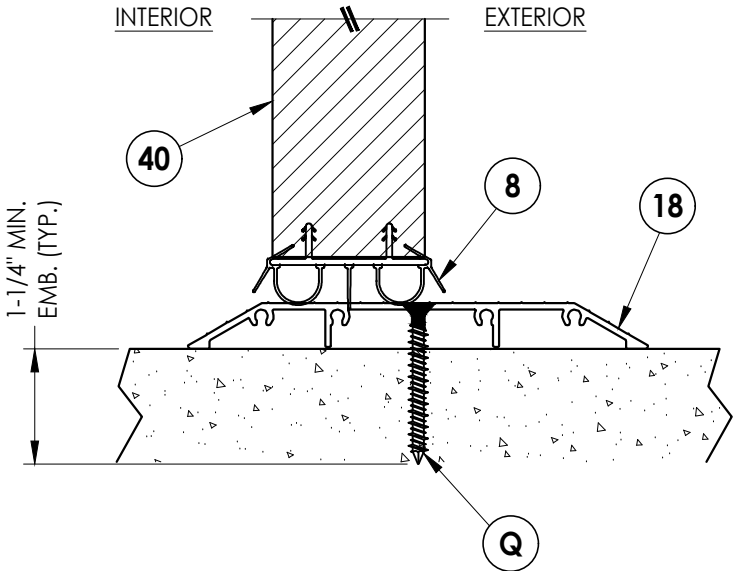
3 6 VERTICAL CROSS SECTION ADA Sill
